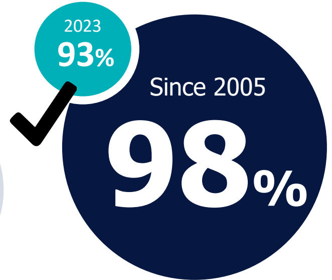
Sulfur Oxides
