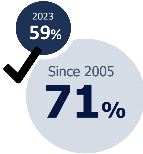
Nitrogen Oxides
